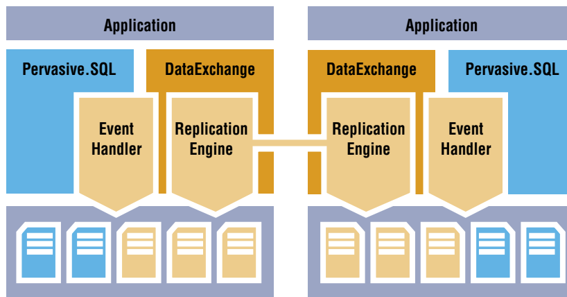
Real-Time Replication with Pervasive DataExchange
